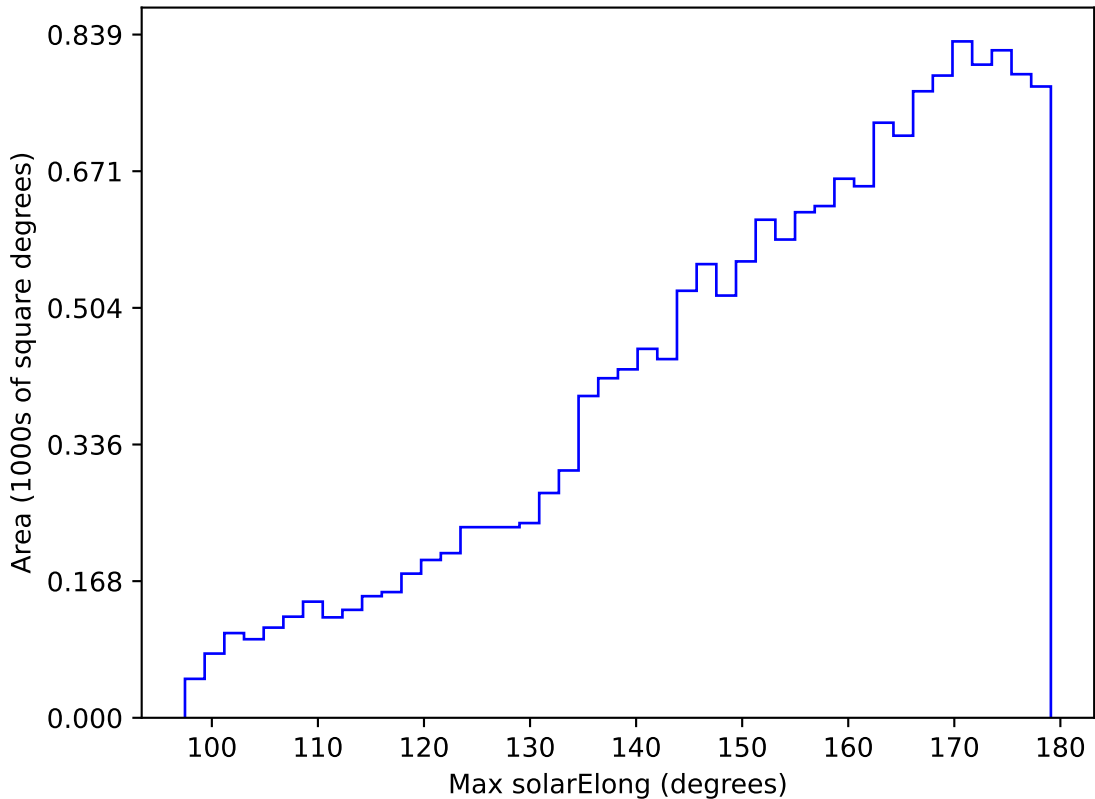
ddf_acor_sf10_lsf20_lsr20_v3.4_10yrs WFD u band: Max solarElong
