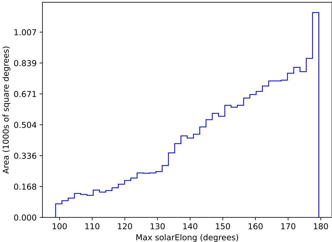
ddf_acor_sf10_lsf20_lsr20_v3.4_10yrs WFD i band: Max solarElong
