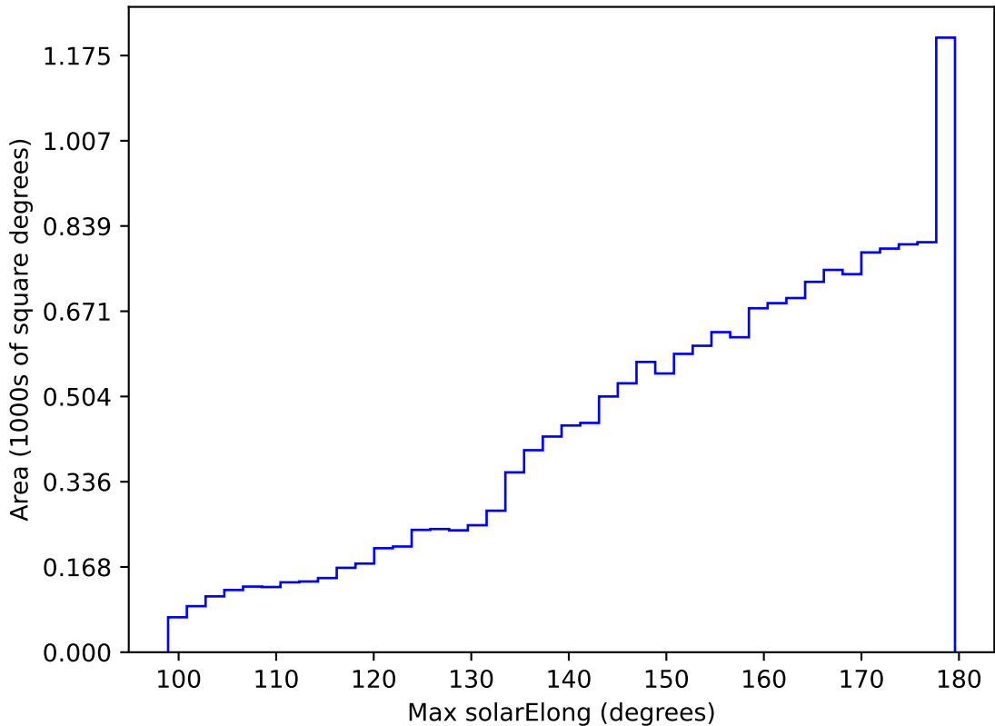
ddf_acor_sf10_lsf20_lsr20_v3.4_10yrs WFD all bands: Max solarElong
