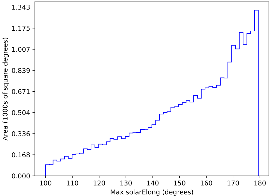
ddf_acor_sf10_lsf20_lsr20_v3.4_10yrs All sky i band: Max solarElong
