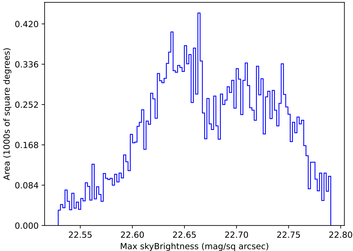
ddf_acor_sf10_lsf20_lsr20_v3.4_10yrs Yr 1 u band: Max skyBrightness
