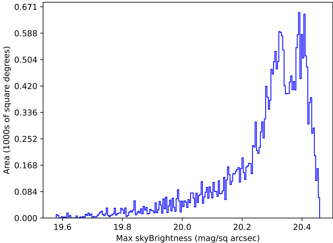
ddf_acor_sf10_lsf20_lsr20_v3.4_10yrs Yr 1 i band: Max skyBrightness
