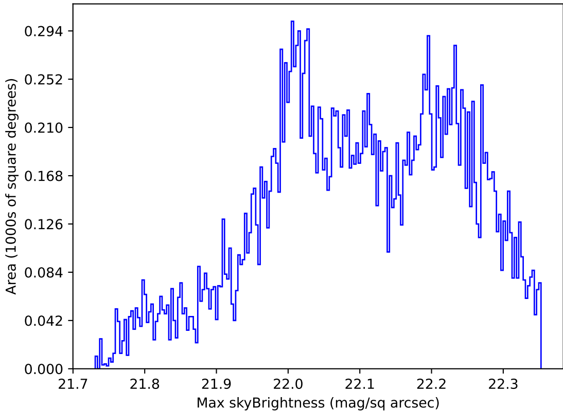
ddf_acor_sf10_lsf20_lsr20_v3.4_10yrs Yr 1 g band: Max skyBrightness
