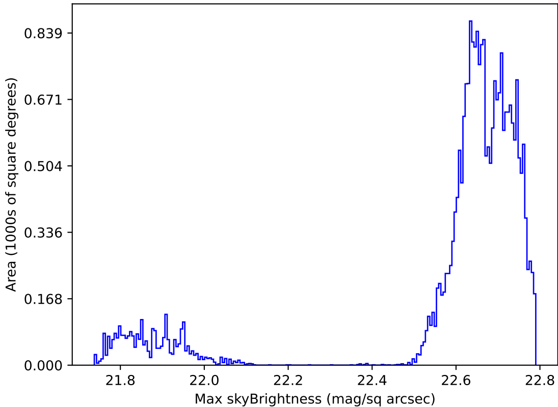
ddf_acor_sf10_lsf20_lsr20_v3.4_10yrs Yr 1 all bands: Max skyBrightness
