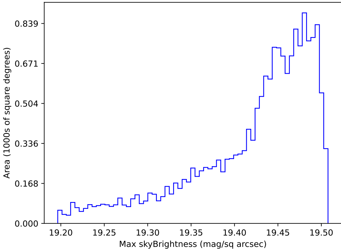
ddf_acor_sf10_lsf20_lsr20_v3.4_10yrs WFD z band: Max skyBrightness
