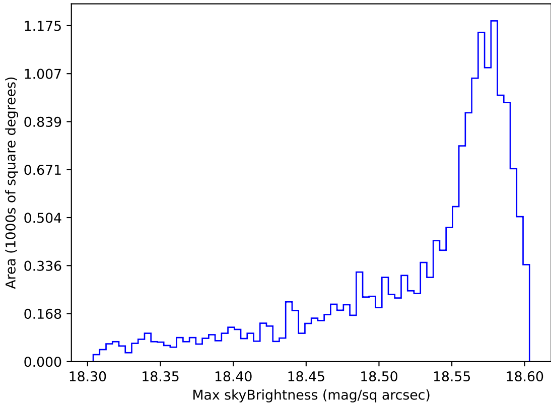
ddf_acor_sf10_lsf20_lsr20_v3.4_10yrs WFD y band: Max skyBrightness
