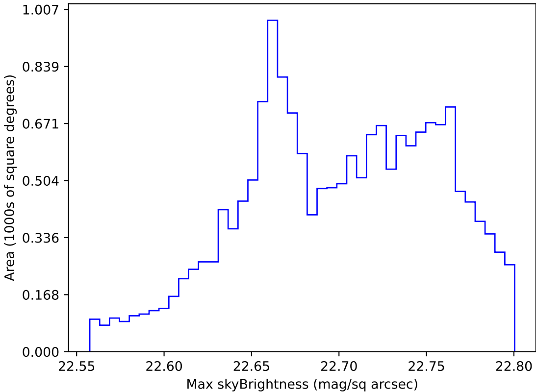
ddf_acor_sf10_lsf20_lsr20_v3.4_10yrs WFD u band: Max skyBrightness
