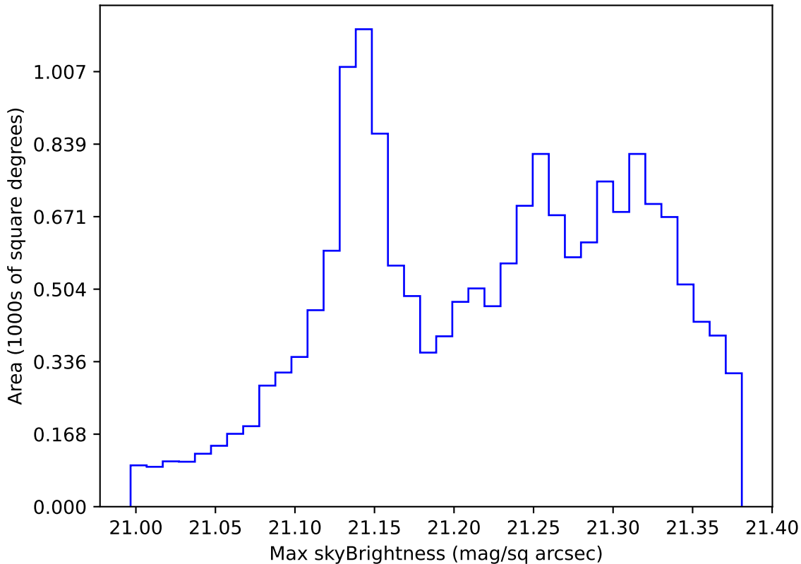
ddf_acor_sf10_lsf20_lsr20_v3.4_10yrs WFD r band: Max skyBrightness
