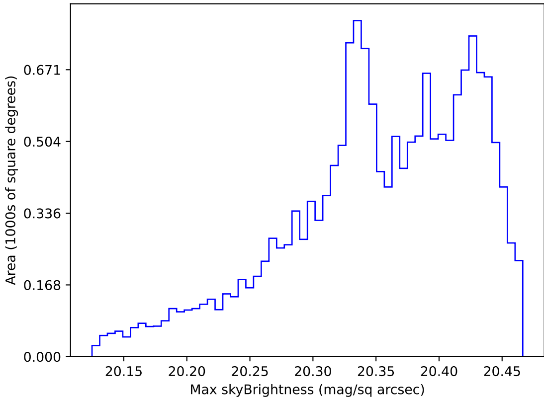
ddf_acor_sf10_lsf20_lsr20_v3.4_10yrs WFD i band: Max skyBrightness
