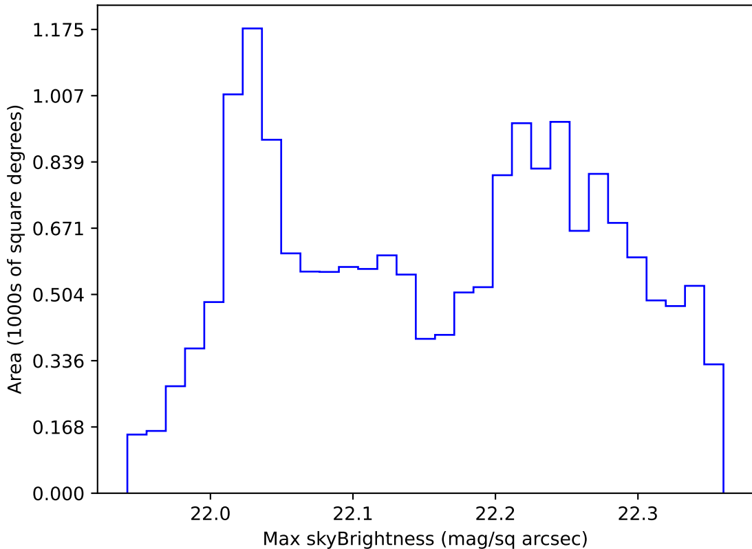
ddf_acor_sf10_lsf20_lsr20_v3.4_10yrs WFD g band: Max skyBrightness
