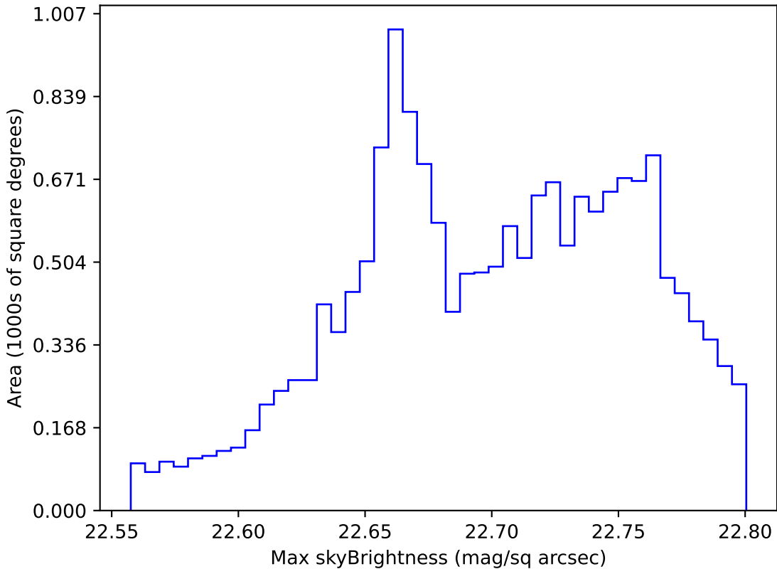
ddf_acor_sf10_lsf20_lsr20_v3.4_10yrs WFD all bands: Max skyBrightness
