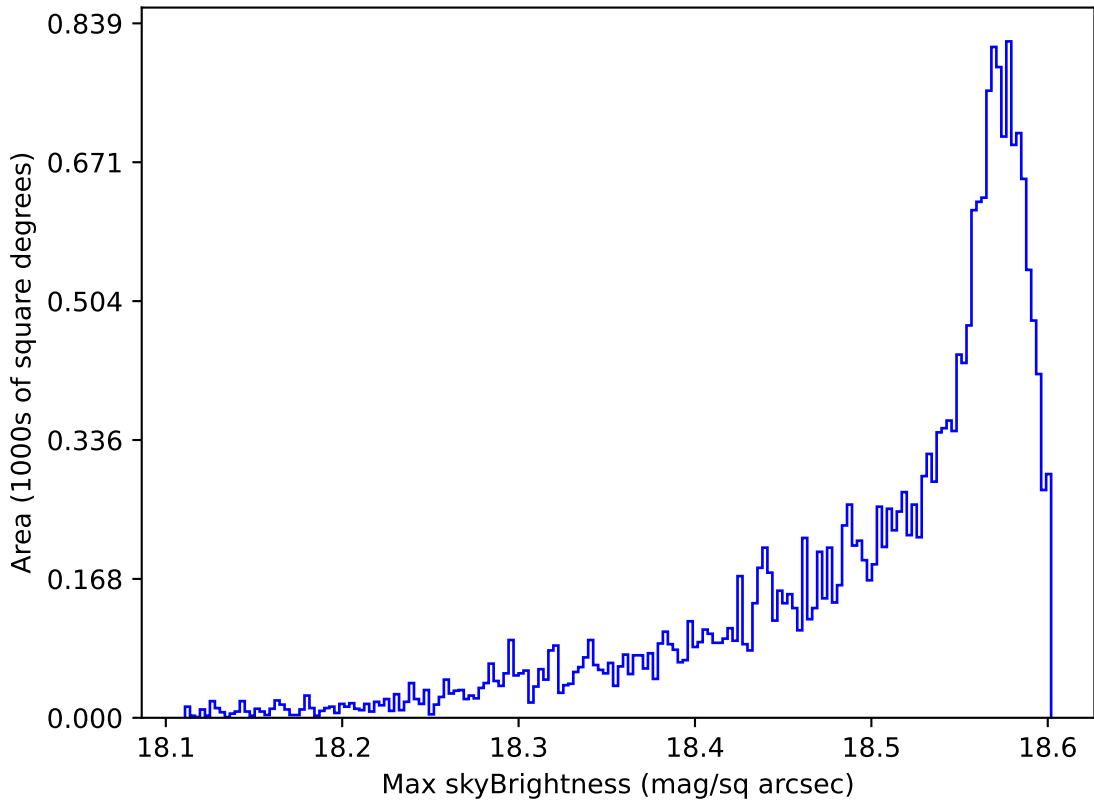
ddf_acor_sf10_lsf20_lsr20_v3.4_10yrs All sky y band: Max skyBrightness
