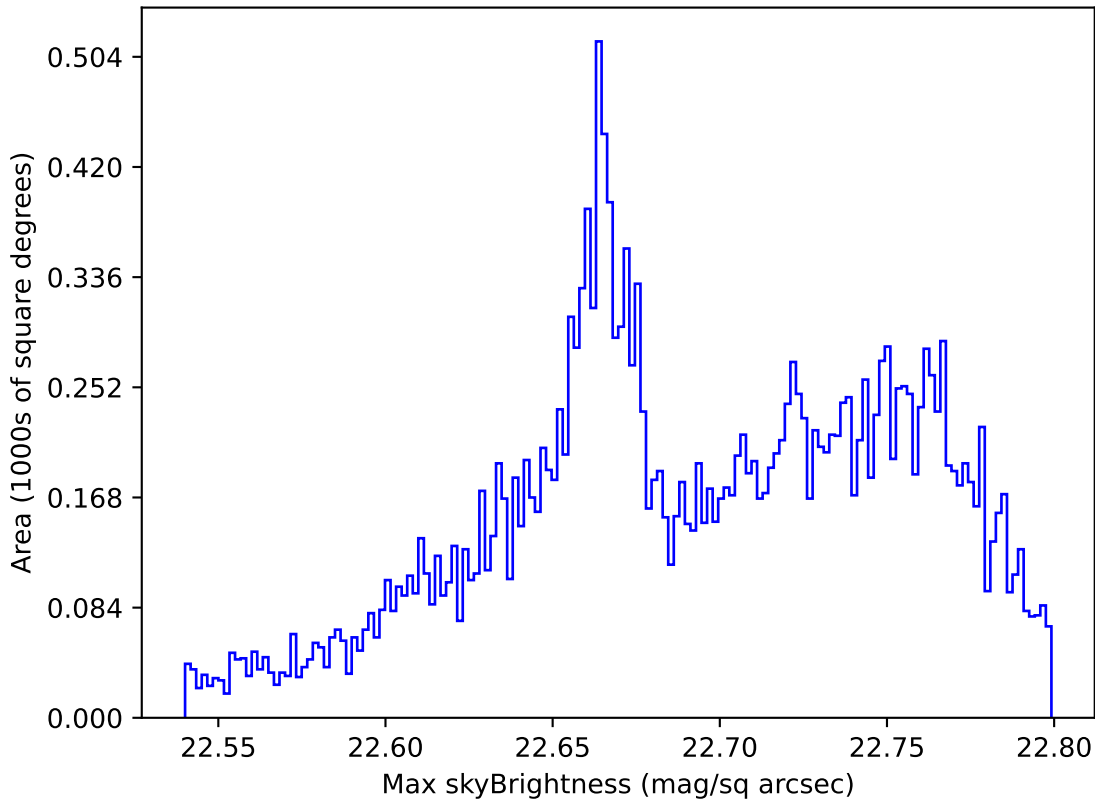
ddf_acor_sf10_lsf20_lsr20_v3.4_10yrs All sky u band: Max skyBrightness
