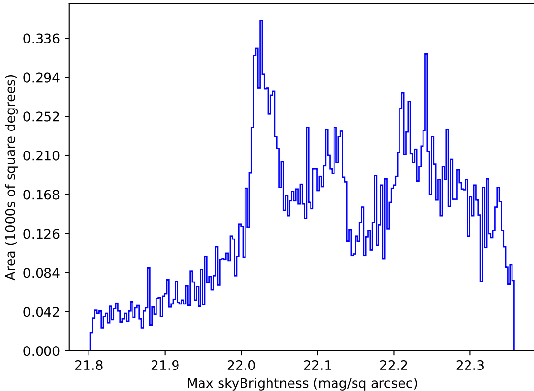
ddf_acor_sf10_lsf20_lsr20_v3.4_10yrs All sky g band: Max skyBrightness
