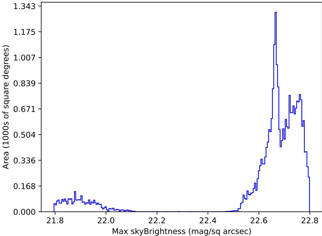
ddf_acor_sf10_lsf20_lsr20_v3.4_10yrs All sky all bands: Max skyBrightness
