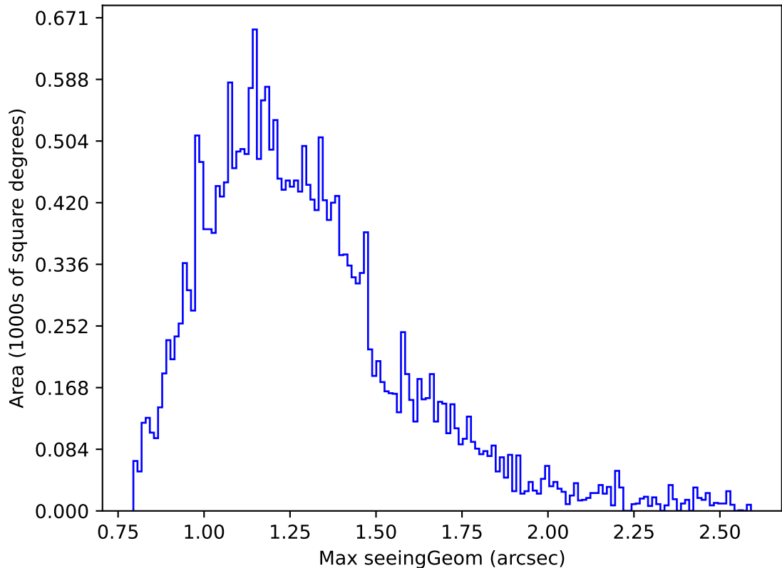
ddf_acor_sf10_lsf20_lsr20_v3.4_10yrs Yr 1 z band: Max seeingGeom
