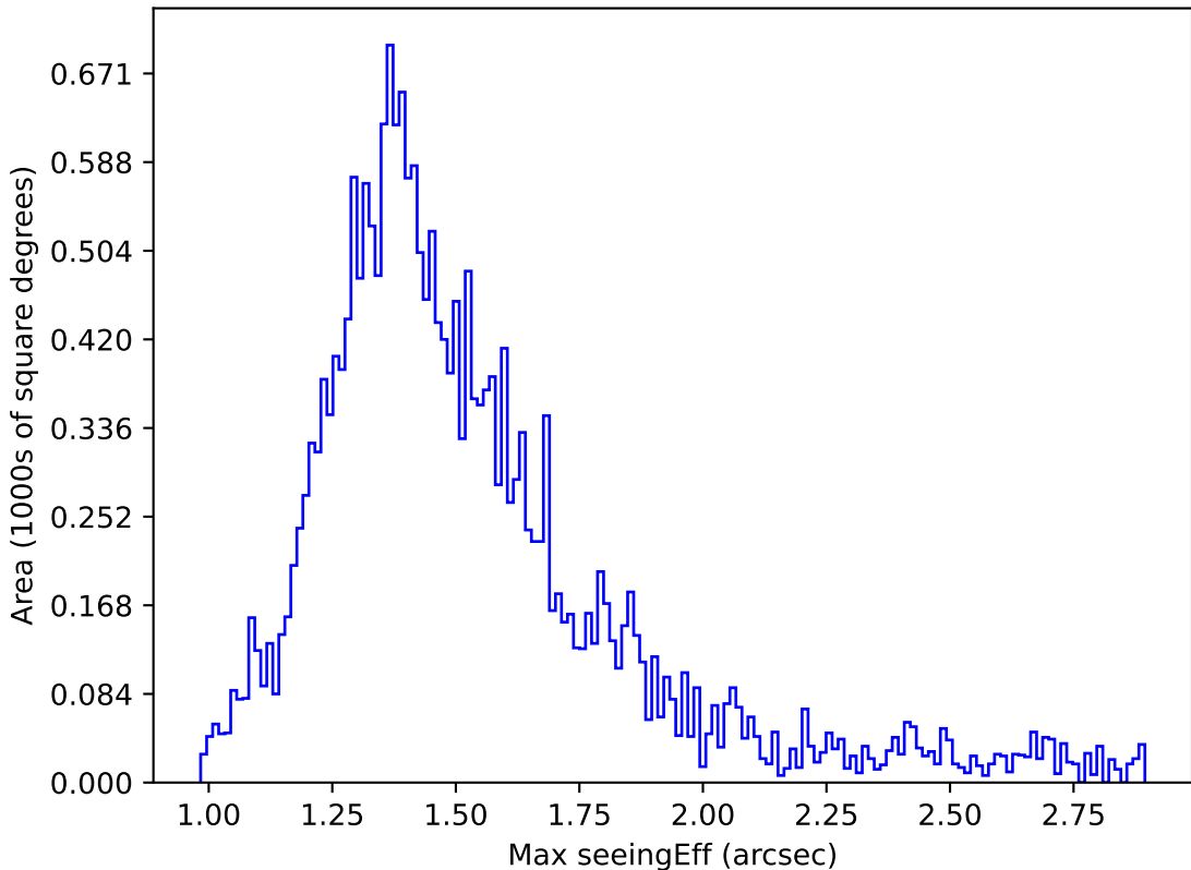
ddf_acor_sf10_lsf20_lsr20_v3.4_10yrs Yr 1 y band: Max seeingEff
