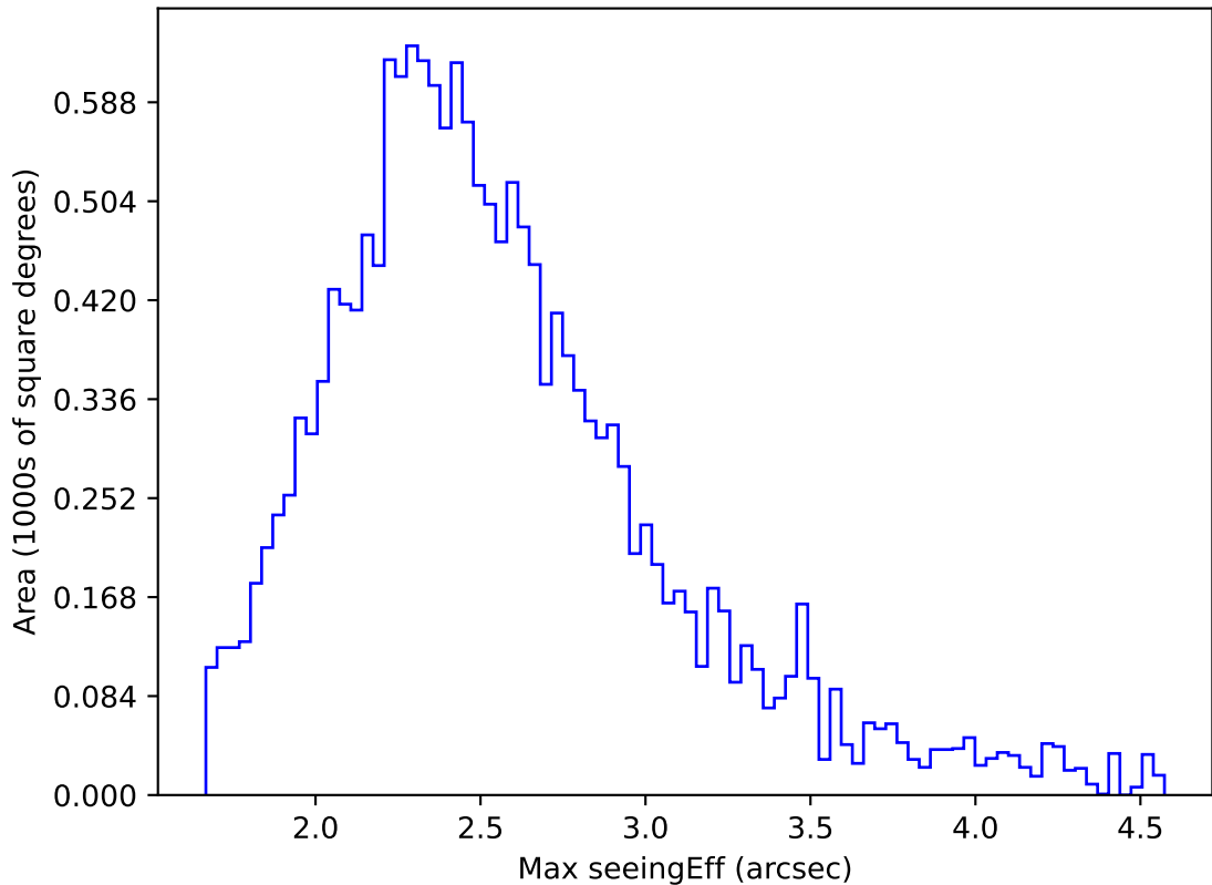
ddf_acor_sf10_lsf20_lsr20_v3.4_10yrs WFD z band: Max seeingEff
