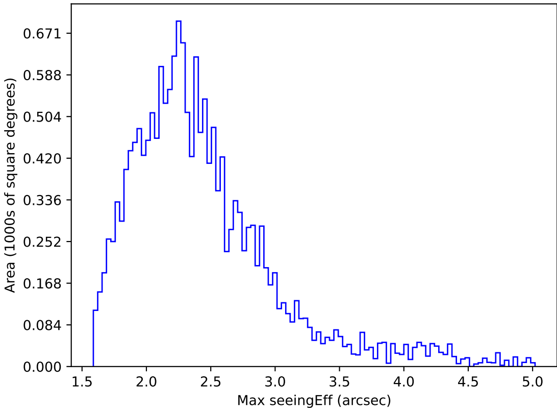
ddf_acor_sf10_lsf20_lsr20_v3.4_10yrs WFD y band: Max seeingEff
