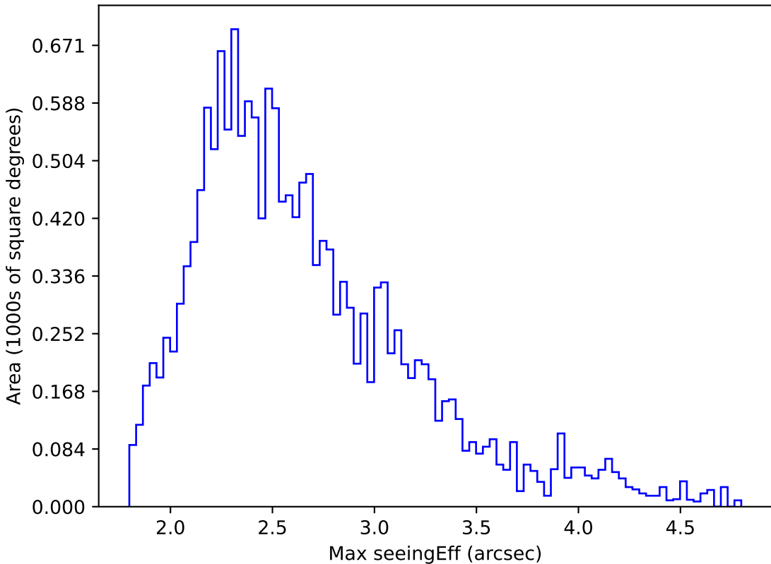
ddf_acor_sf10_lsf20_lsr20_v3.4_10yrs WFD r band: Max seeingEff
