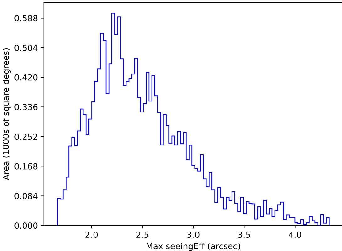
ddf_acor_sf10_lsf20_lsr20_v3.4_10yrs WFD g band: Max seeingEff
