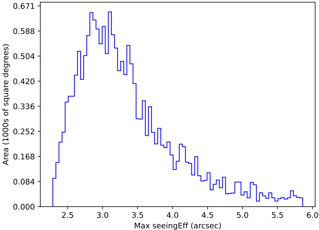
ddf_acor_sf10_lsf20_lsr20_v3.4_10yrs WFD all bands: Max seeingEff
