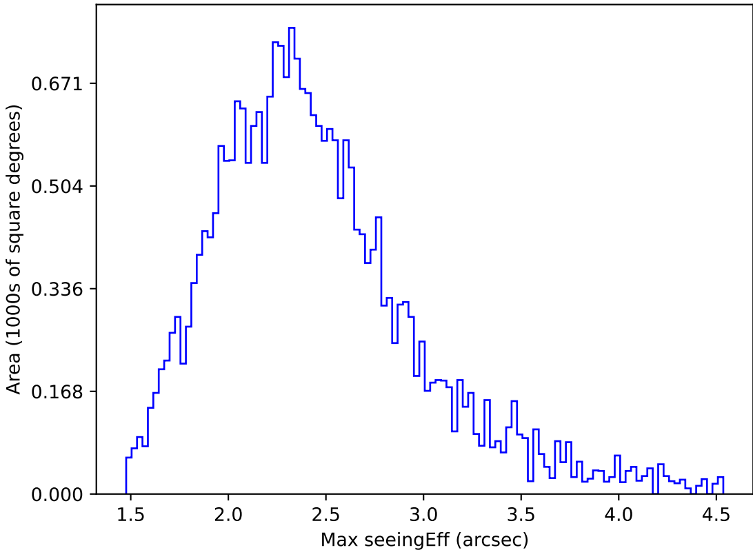
ddf_acor_sf10_lsf20_lsr20_v3.4_10yrs All sky z band: Max seeingEff
