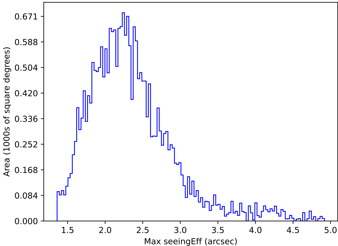
ddf_acor_sf10_ls20_lsr20_v3.4_10yrs All sky y band: Max seeingEff
