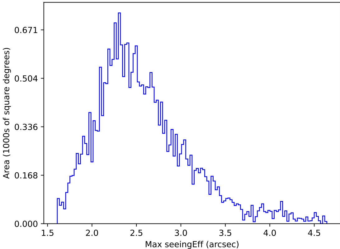
ddf_acor_sf10_lsf20_lsr20_v3.4_10yrs All sky r band: Max seeingEff
