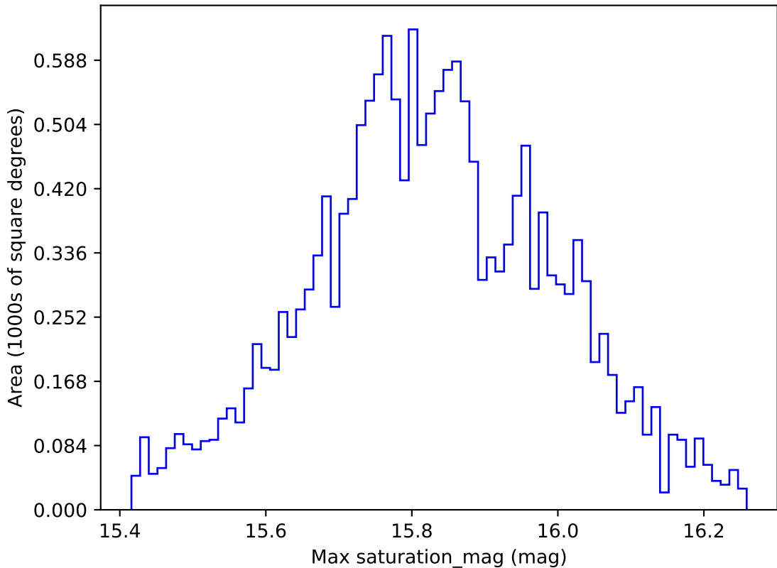
ddf_acor_sf10_lsf20_lsr20_v3.4_10yrs WFD all bands: Max saturation_mag
