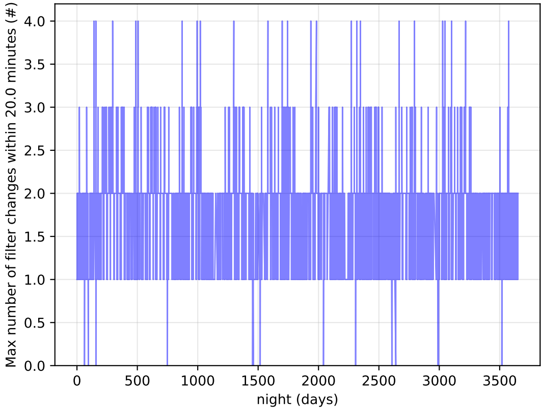
ddf_acor_sf10_Isf20_Isr20_v3.4_10yrs Per Night: Max number of filter changes within 20.0 minutes
