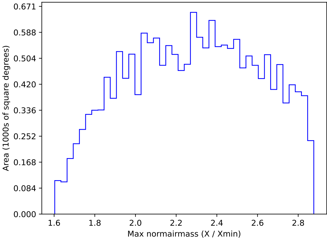
ddf_acor_sf10_lsf20_lsr20_v3.4_10yrs WFD i band: Max normairmass
