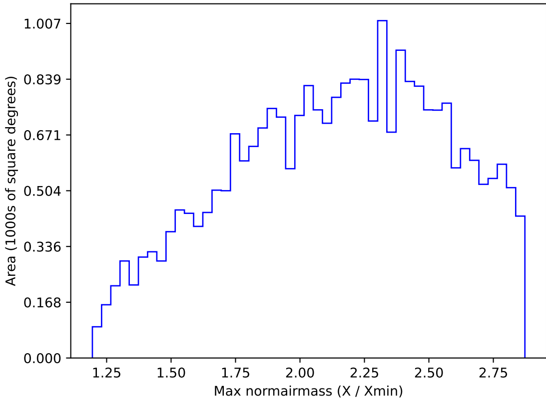
ddf_acor_sf10_lsf20_lsr20_v3.4_10yrs All sky z band: Max normairmass
