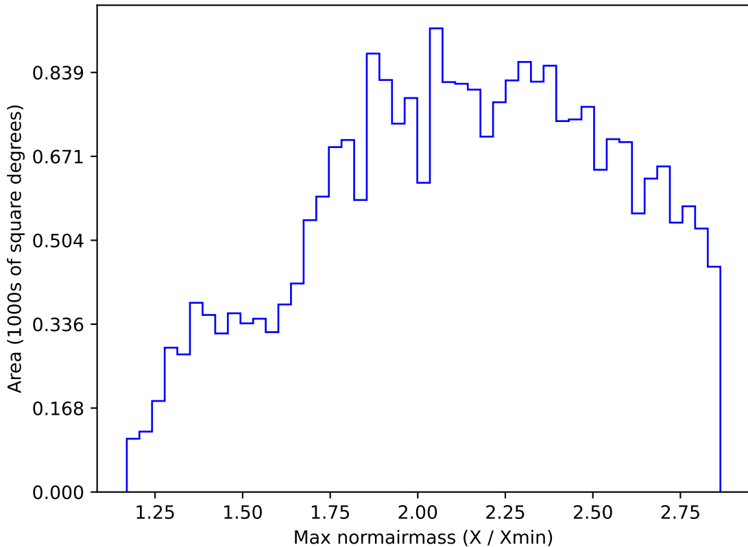
ddf_acor_sf10_lsf20_lsr20_v3.4_10yrs All sky i band: Max normairmass
