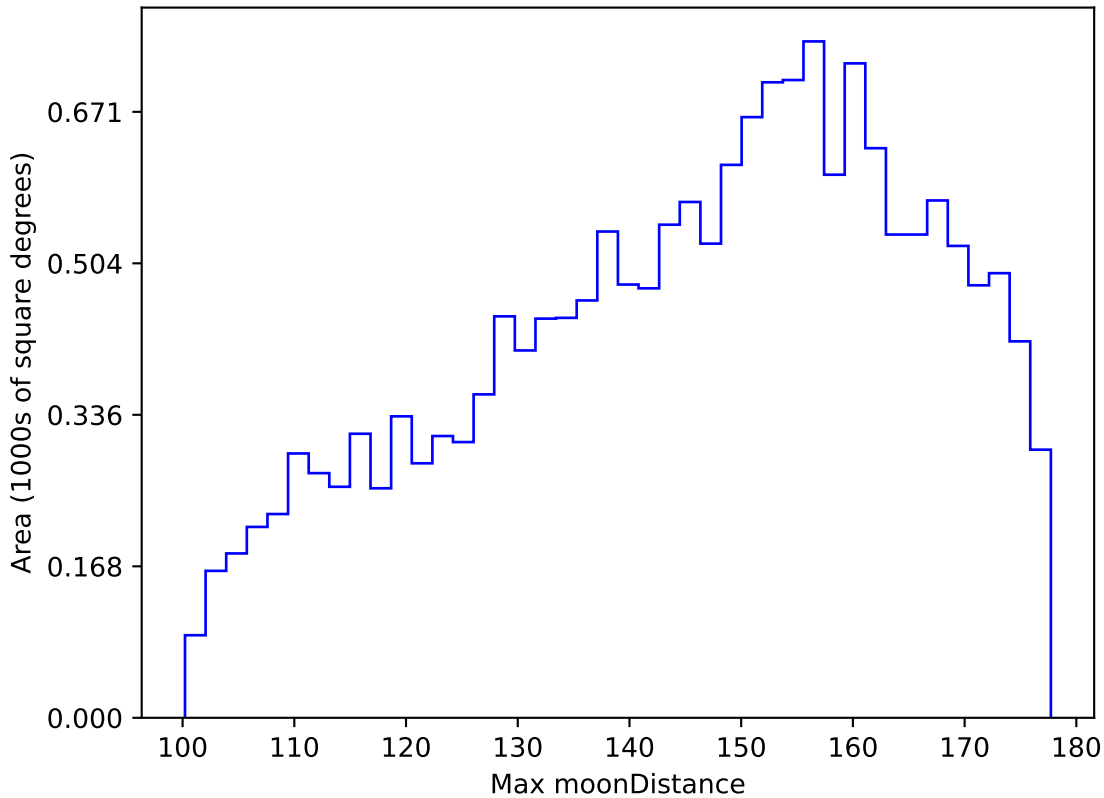
ddf_acor_sf10_lsf20_lsr20_v3.4_10yrs WFD y band: Max moonDistance
