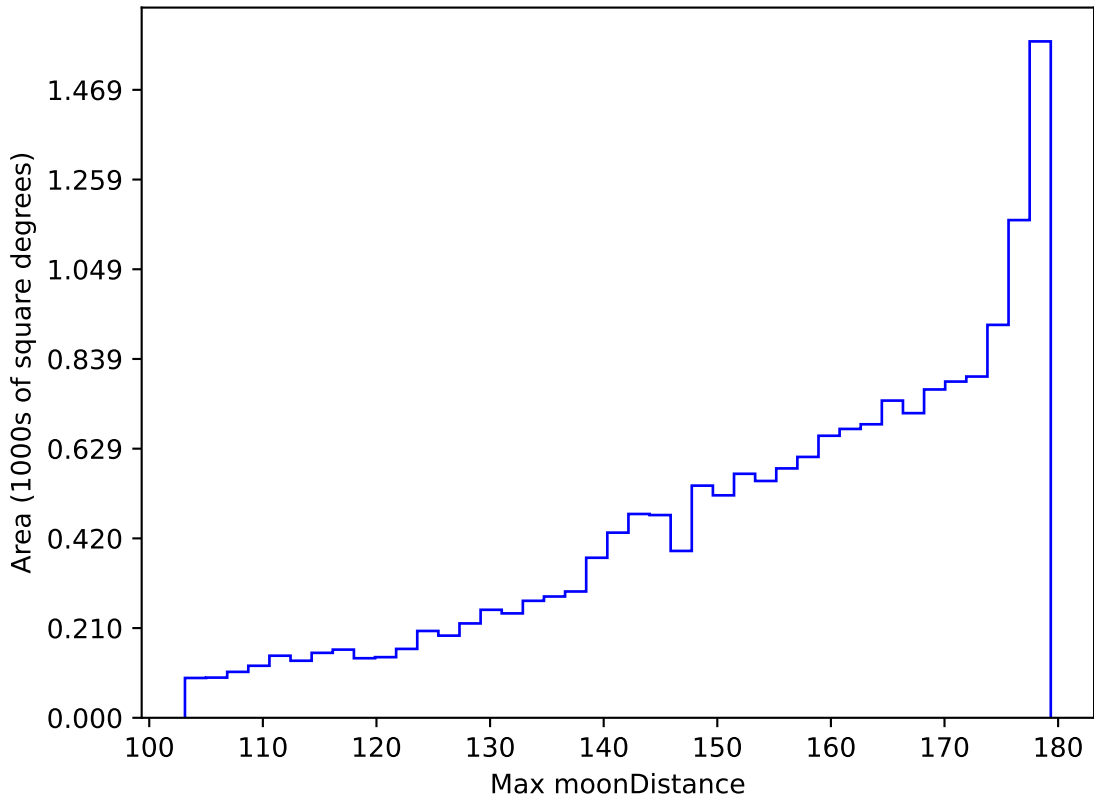
ddf_acor_sf10_lsf20_lsr20_v3.4_10yrs WFD r band: Max moonDistance
