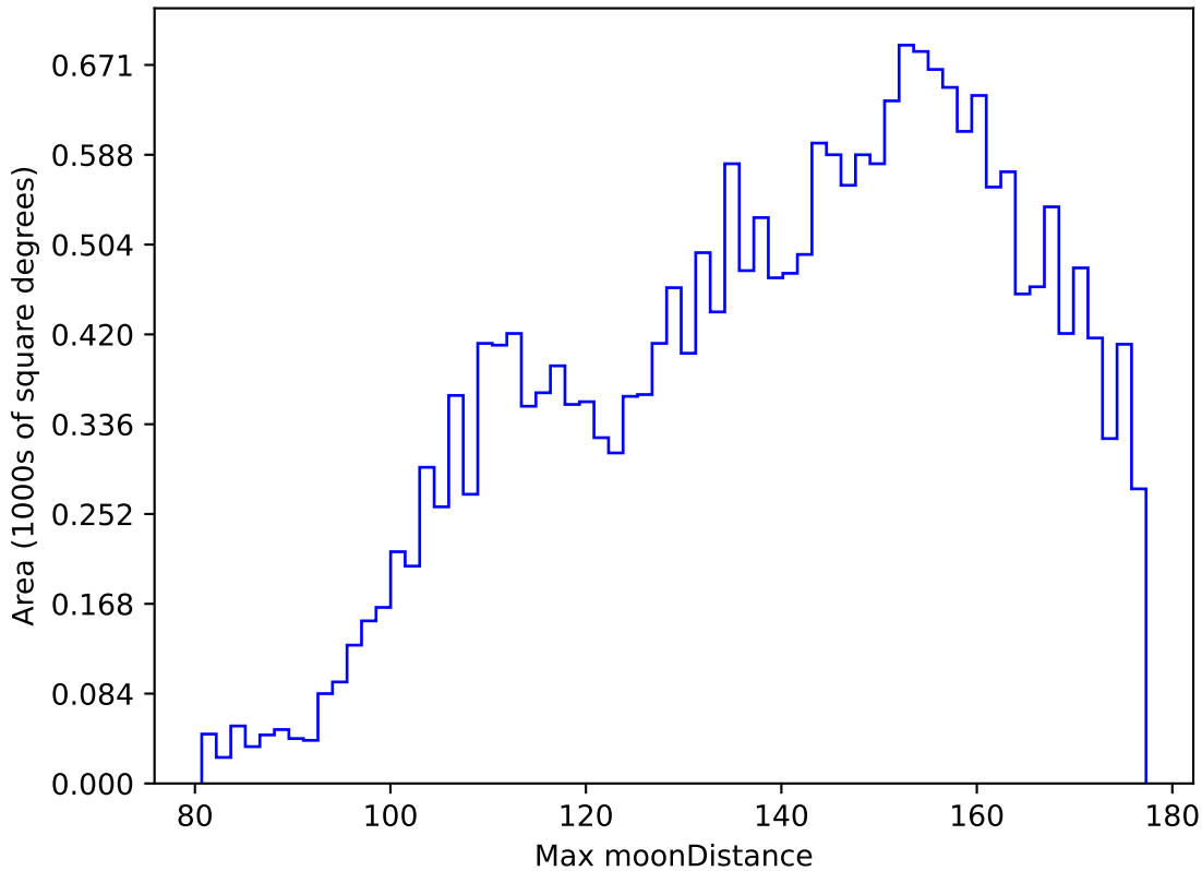
ddf_acor_sf10_lsf20_lsr20_v3.4_10yrs All sky y band: Max moonDistance
