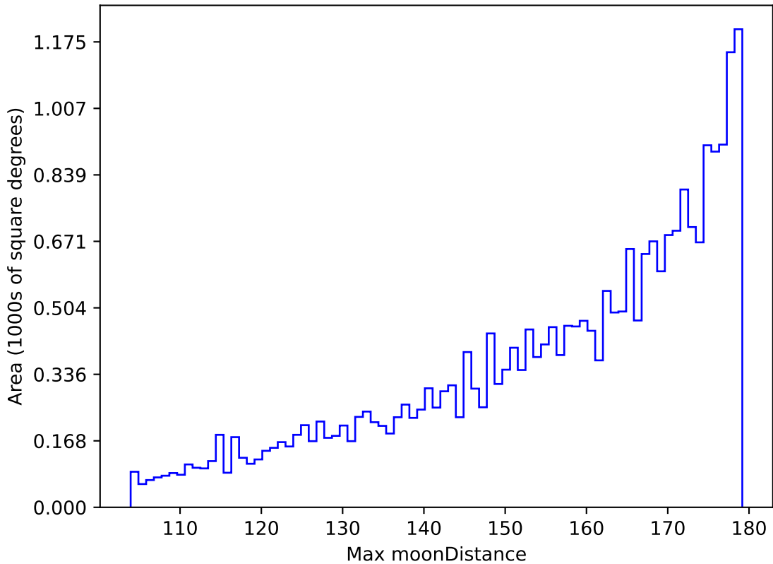
ddf_acor_sf10_lsf20_lsr20_v3.4_10yrs All sky r band: Max moonDistance
