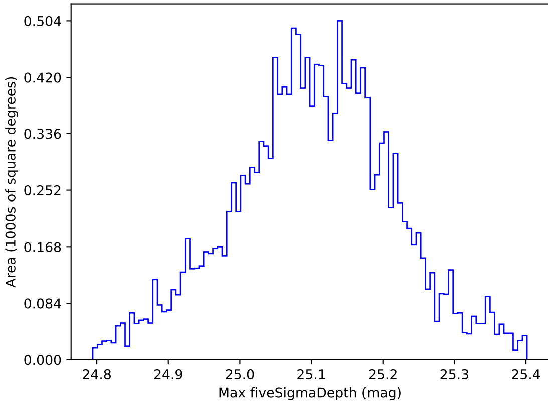
ddf_acor_sf10_lsf20_lsr20_v3.4_10yrs WFD g band: Max fiveSigmaDepth
