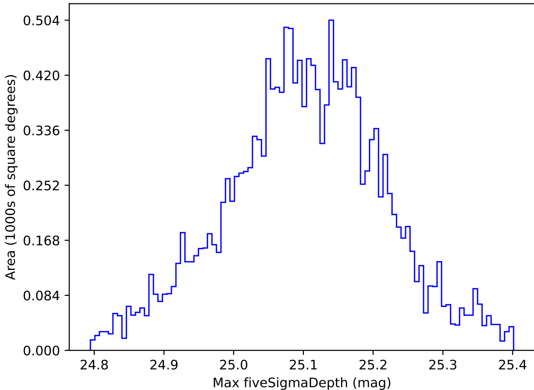
ddf_acor_sf10_lsf20_lsr20_v3.4_10yrs WFD all bands: Max fiveSigmaDepth
