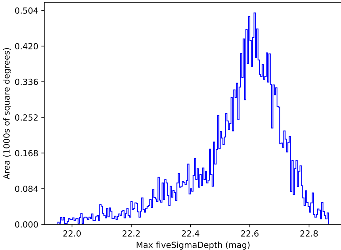
ddf_acor_sf10_ls20_lsr20_v3.4_10yrs All sky y band: Max fiveSigmaDepth
