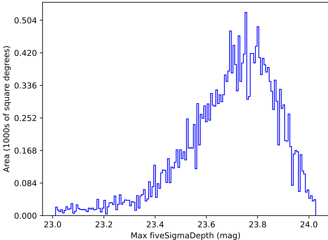
ddf_acor_sf10_lsf20_lsr20_v3.4_10yrs All sky u band: Max fiveSigmaDepth
