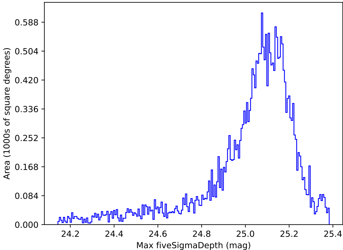
ddf_acor_sf10_lsf20_lsr20_v3.4_10yrs All sky g band: Max fiveSigmaDepth
