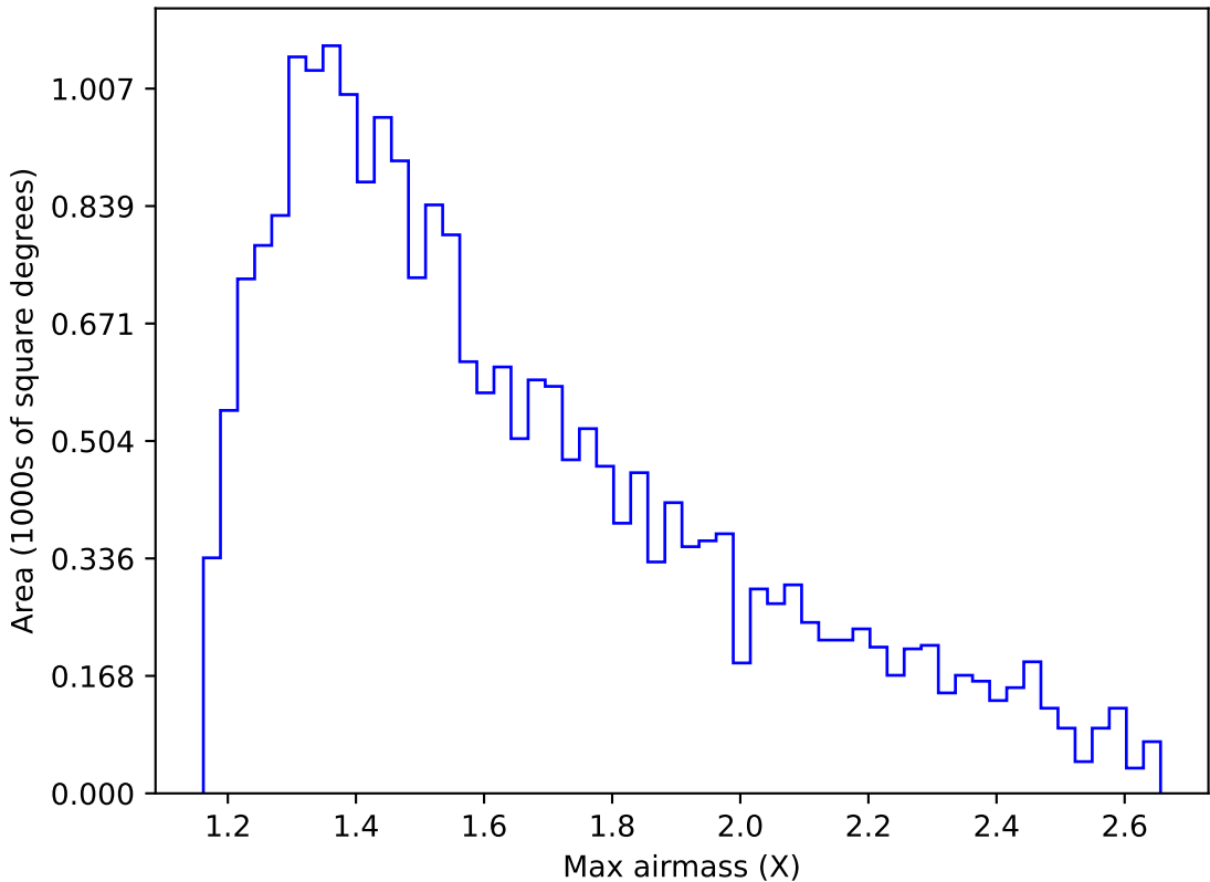
ddf_acor_sf10_lsf20_lsr20_v3.4_10yrs Yr 1 y band: Max airmass
