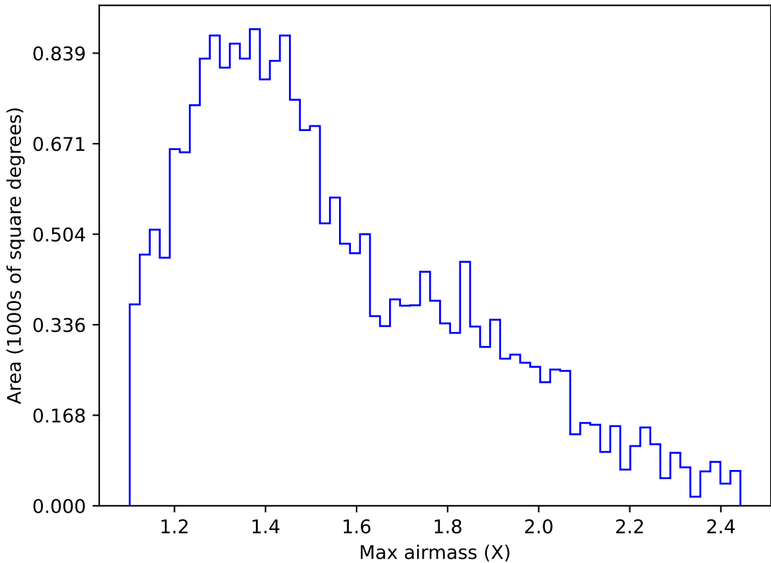
ddf_acor_sf10_lsf20_lsr20_v3.4_10yrs Yr 1 u band: Max airmass
