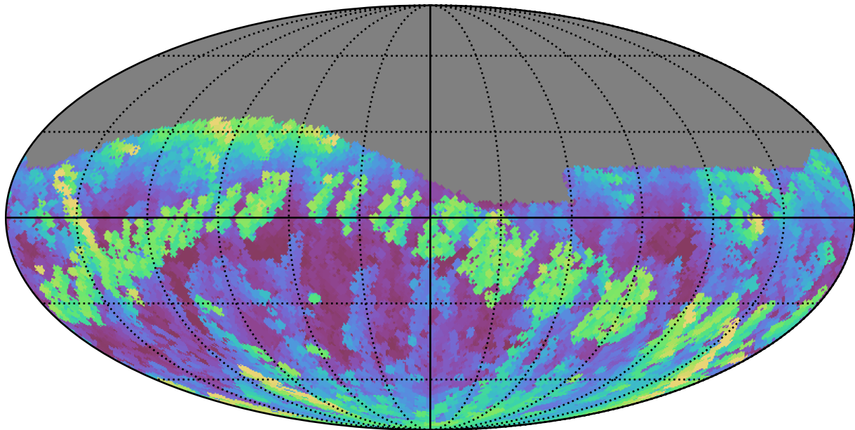
ddf_acor_sf10_lsf20_lsr20_v3.4_10yrs Yr 1 r band: Max airmass
