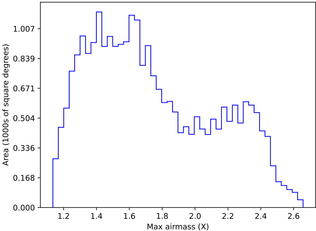
ddf_acor_sf10_lsf20_lsr20_v3.4_10yrs Yr 1 r band: Max airmass
