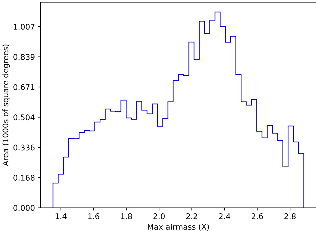
ddf_acor_sf10_lsf20_lsr20_v3.4_10yrs Yr 1 all bands: Max airmass
