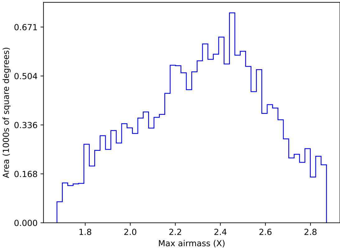
ddf_acor_sf10_lsf20_lsr20_v3.4_10yrs WFD y band: Max airmass
