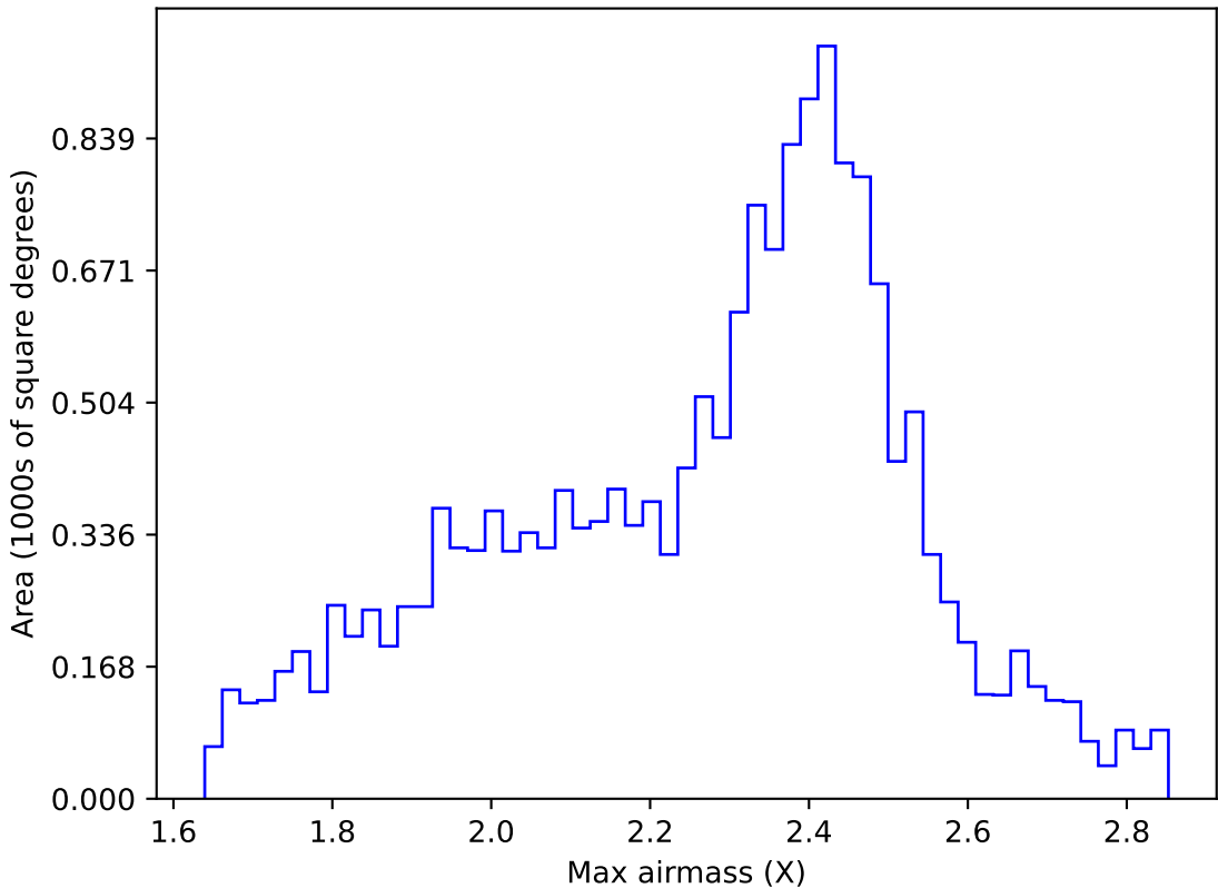
ddf_acor_sf10_lsf20_lsr20_v3.4_10yrs WFD r band: Max airmass
